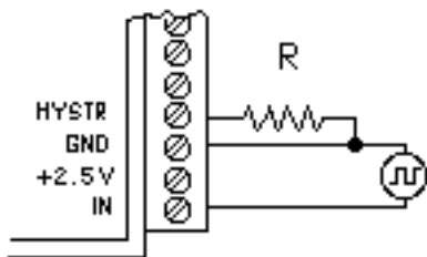
Figure B-4. Controlling Switching Level and Hysteresis.
