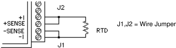
Figure C-3. 2-Wire RTD Configuration.
